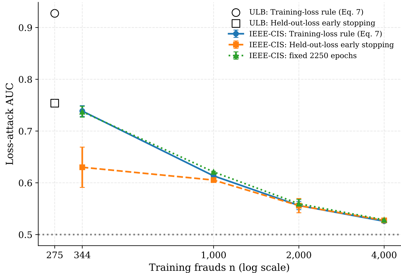
(b) Leakage against data scale
