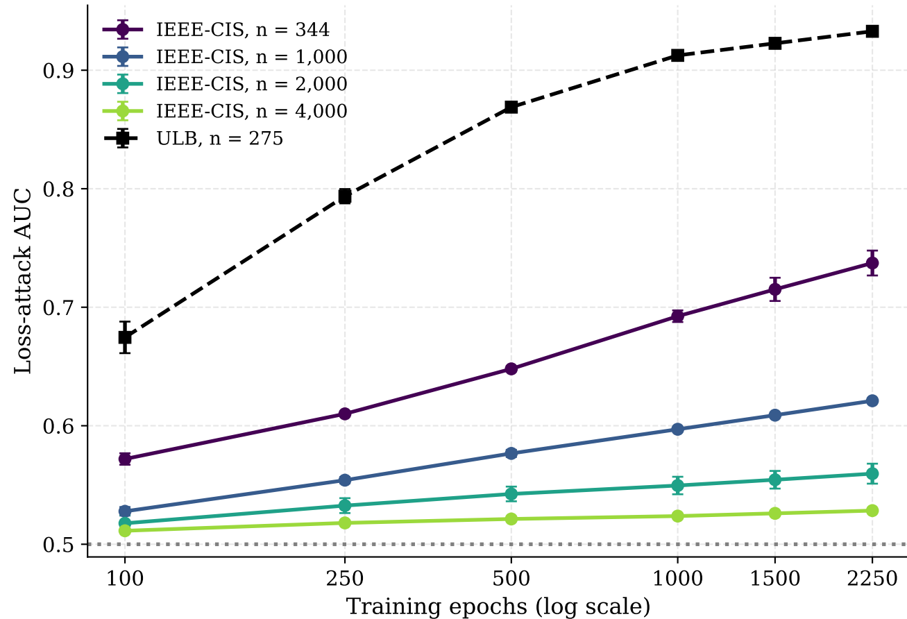
(a) Leakage against training length
